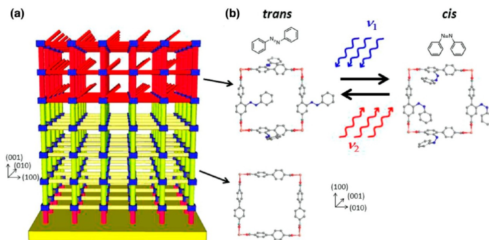
Figure 9. Structural drawing of heteroepitaxial two-component MOF: the photounactive \text{Cu}_2(\text{bpdcc})_2(\text{bipy}) SURMOF (yellow) is grown on the pretreated gold substrate, and the photoresponsive \text{Cu}_2(\text{ab-bpdcc})_2(\text{bipy}) SURMOF (red) containing photoswitchable azobenzene is grown on top (a). View of the pore window in the [001] direction (b). Reproduced from ref 103. Copyright 2014 American Chemical Society.
