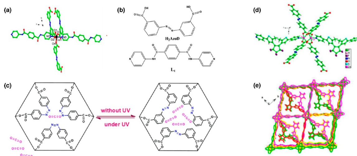
Figure 7. Schematic view of Gen-3 MOF unit structure. \text{Co}_2\text{L}_2(\text{AzoD})_2 \cdot 2\text{DMF} : the simplest MBU (a), the ligands (b), and photoinduced structural changes in the MOF cage (c). Reprinted in part with permission from ref 96. Copyright 2016 Taylor & Francis. \text{Zn}(\text{AzDC})\text{L}_{0.5} \cdot (\text{DMF})_{1.5} : the paddle-wheel MBU (d) and the 3D framework (e). Reprinted in part with permission from ref 97. Copyright 2017 The Royal Society of Chemistry.
